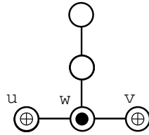
Figure 3: The graph induced by an equivalence class may be disconnected - u and v are in the same equivalence class, different from the one w belongs to.
