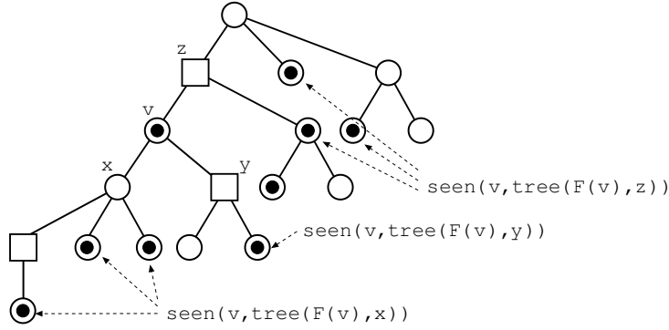
Figure 4: \text{seen}(v)
