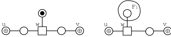
Figure 6: Lemma 6.11, condition 1. F_1 = R(F(w), u) \cap R(F(w), v)
