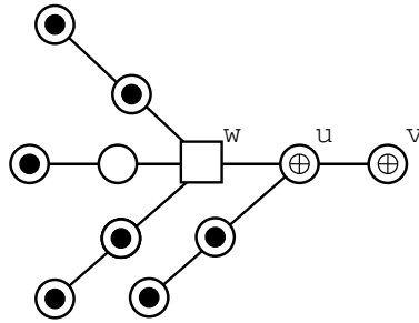
Figure 10: Example for the proof of Lemma 6.11, case 1 (b) i A
