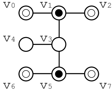
Figure 15: An instance of 2-PM
