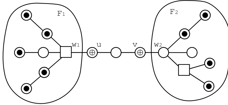
Figure 5: u and v are not equivalent
