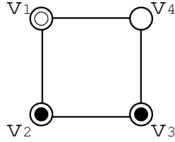
Figure 2: A cyclic pebble swap on (v_1, v_2, v_3) is a (v_1, v_2) color swap.
