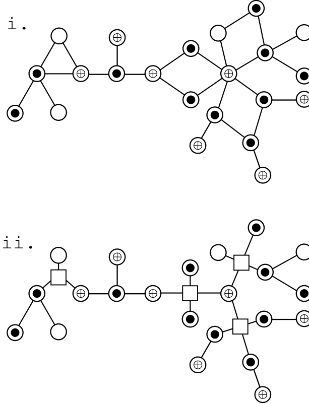
Figure 13: Converting G (i) into G_T (ii)
