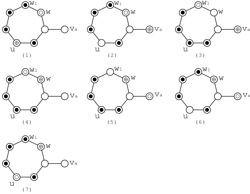
Figure 14: Swapping pebbles w and u on a cycle with an attached edge. To help follow the steps, the swapped pebbles are marked with different texture.
