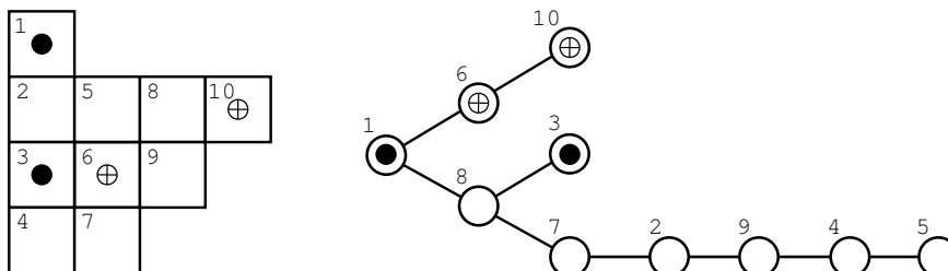
Figure 1: Knight Exchange game modeled as a 2-PM on a tree. It is required to exchange the black pebbles with the gray pebbles.
