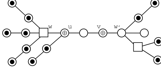
Figure 11: Example for the proof of Lemma 6.11, case 1 (b) i B
