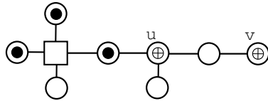
Figure 8: Lemma 6.11, condition 4.
