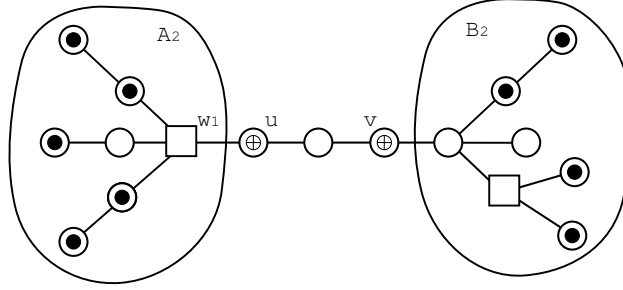
Figure 9: Example for the proof of Lemma 6.11, case 1 (a)
