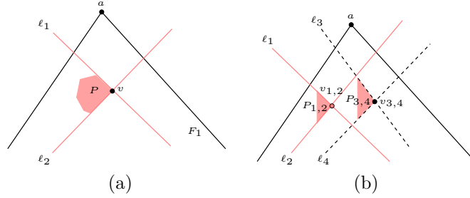
Figure 3: (a) The cross section of a cell of \mathcal{A}(\mathcal{H}) on F_1 , and the pair of lines \ell_1, \ell_2 that it charges. (b) The vertices v_{1,2} and v_{3,4} cannot both be edges of G , because the polygon P_{3,4} (partially highlighted) is fully contained in the wedge spanned by the respective planes containing \ell_1, \ell_2 (and opposite to the wedge that contains P_{1,2} ), which meets only two facets of W .
