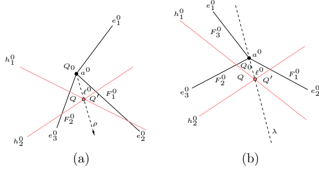
Figure 2: The proof of Lemma 2.2.
