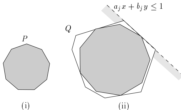
Figure 1: (i) The polygon P ; (ii) The polygon Q and a largest copy of P inside Q
