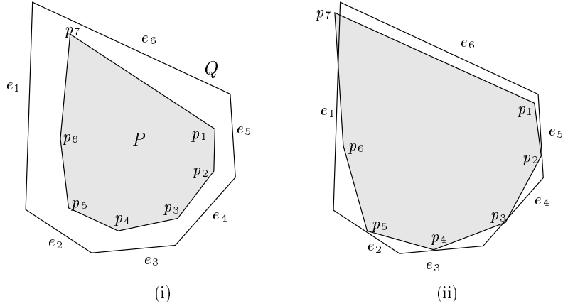
Figure 3: Spurious facets generated by the algorithm: (i) The orientation of P lies in K_{i-1} , where \xi_i = w_{2,5} ; (ii) A placement of P corresponding to a spurious facet of S_{i-1} \cup \{w_{2,5}\} .
