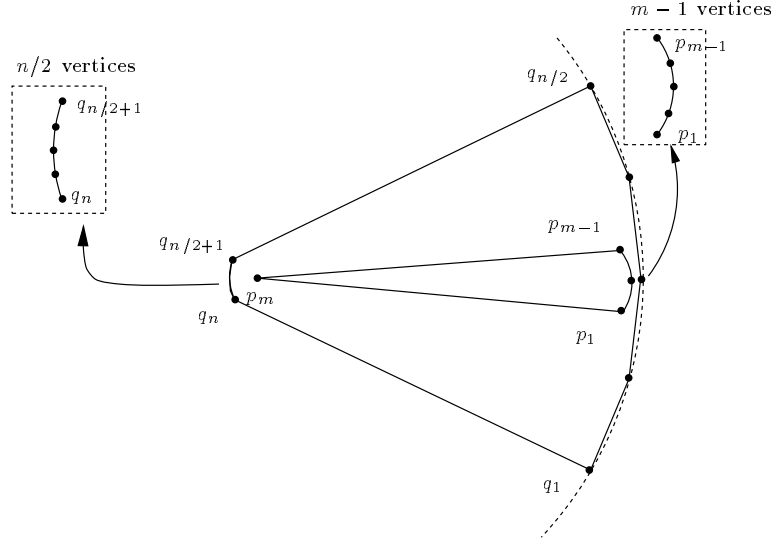
Figure 4: Polygons P and Q for which there exist \Omega(mn^2) similar placements of P in Q with four vertex-edge incidences per placement
