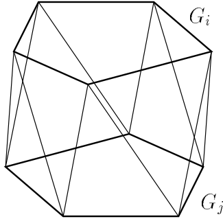
Figure 2: Convex hull of parallel polygons
