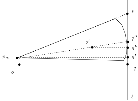
Figure 5: Proof of claim
