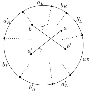
Figure 7: Partition of the circle \sigma_r into maximal arcs.
