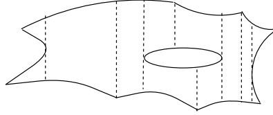
Figure 2: Vertical decomposition: Step II.
