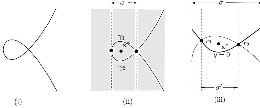
Figure 5: (i) The set \sqrt{\pi} of roots of \pi . (ii) The cylindrical algebraic decomposition of \pi ; (iii) The curves g = 0 and \gamma_1
