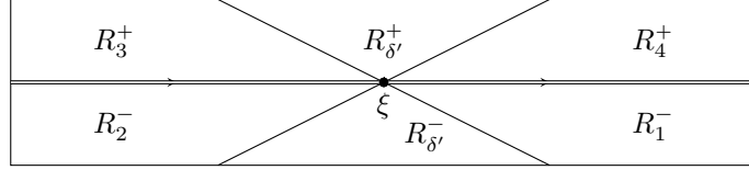
FIGURE 14. The developing image of rectangles when \delta' shrinks to a point and the two singularities coalesce.
