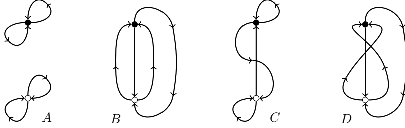
FIGURE 6. List of all maximal horizontal data diagrams in \mathcal{H}(1, 1) up to switching labels and orientations. See Figure 4 for a polygonal presentation of a cylinder decomposition of type A.
