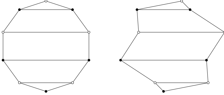
FIGURE 4. Applying \text{Rel}_t (with t > 0 ) to the tipped decagon.
