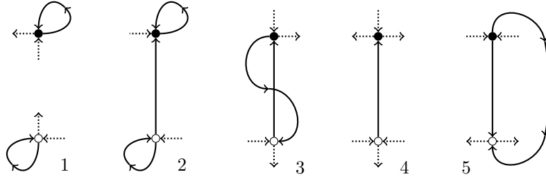
FIGURE 7. These figures represent some non-maximal horizontal data diagrams in \mathcal{H}(1, 1) .
