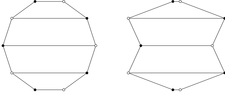
FIGURE 3. Applying \text{Rel}_t (with t < 0 ) to the decagon. When t < -a or t > b then \text{Rel}_t fails to be defined, where a is the length of the top segment and b is the length of the second segment from the top.
