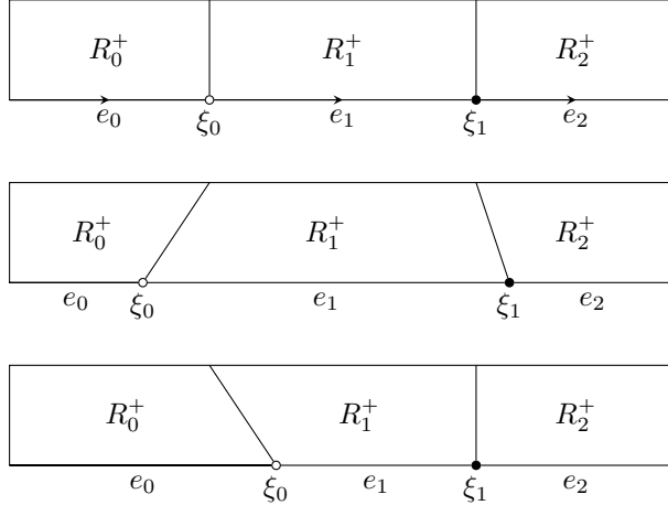
FIGURE 10. The effect of different deformations, transforming the rectangles into trapezoids.
