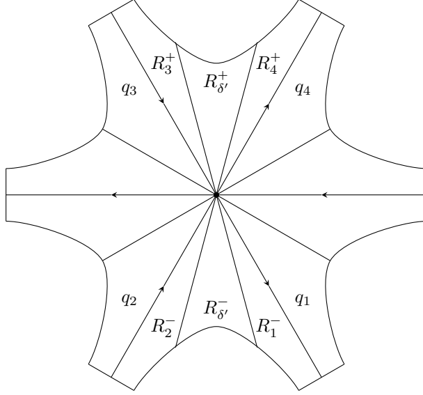
FIGURE 15. The corresponding topologically correct picture. The chosen prong edge is labeled q_1 .
