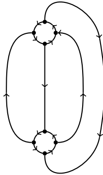
FIGURE 5. A horizontal data diagram on a blown up surface.
