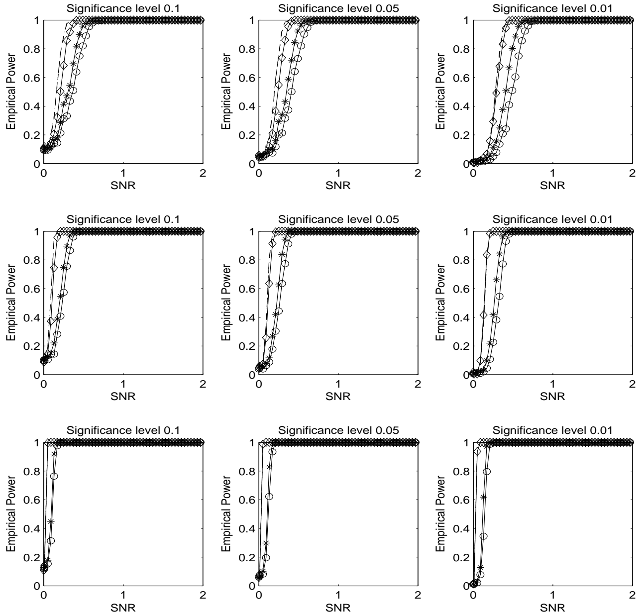
Figure 1: Empirical power for the five tests for the test function m_g , n = 32 (first row), n = 64 (second row), and n = 256 (third row). The dash line refers to the V_d test; the dash-dot line refers to the V_f test; the solid-circle line refers to the M_{2,\alpha} (with order l = 2 ) test; the solid-asterisk line refers to the \hat{T}_n^{(1,2)} (with order l = 1 ) test; the solid-diamond line refers to the A_{min} test.
