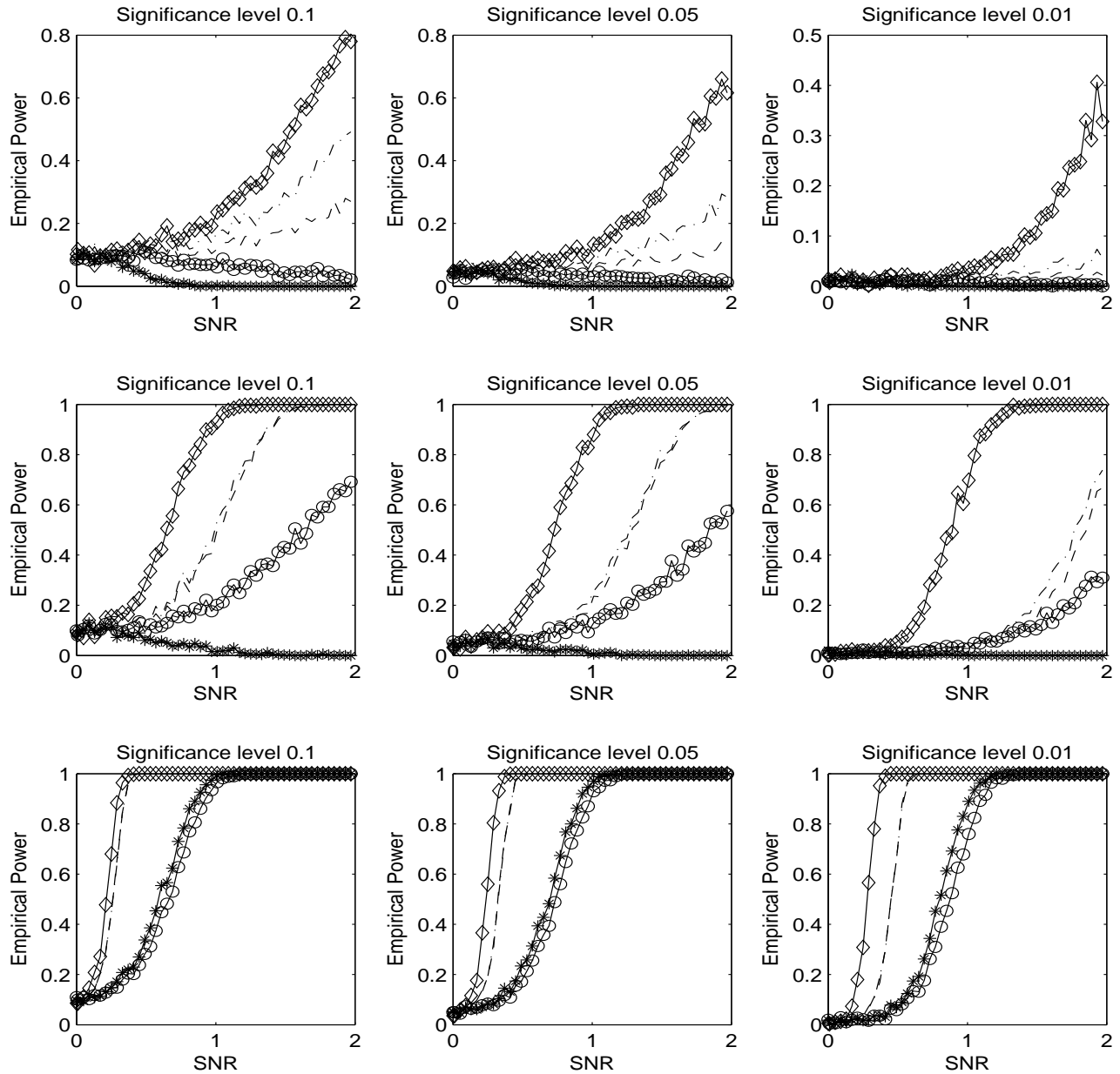
Figure 2: Empirical power for the five tests for the test function m_{13} , n = 32 (first row), n = 64 (second row), and n = 256 (third row). The dash line refers to the V_d test; the dash-dot line refers to the V_f test; the solid-circle line refers to the M_{2,\alpha} (with order l = 2 ) test; the solid-asterisk line refers to the \hat{T}_n^{(1,2)} (with order l = 1 ) test; the solid-diamond line refers to the A_{min} test.
