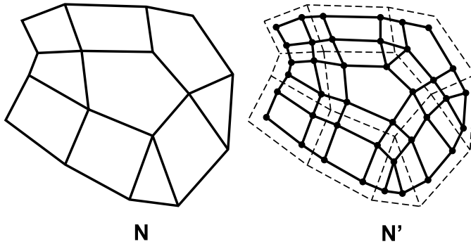
Figure 3.13. Dual-type refinement
