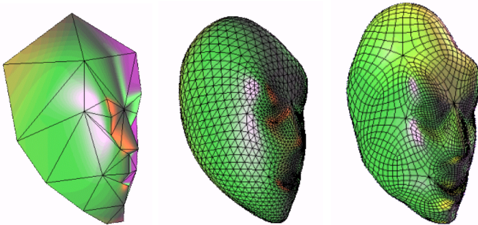
Figure 3.12. Head: initial control net (left), two iterations with the Loop scheme (middle) and with the Catmull–Clark scheme (right)
