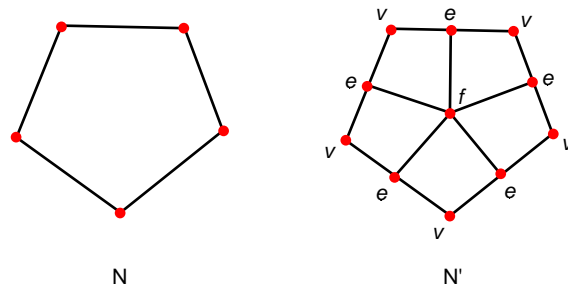
Figure 3.10. Primal-type refinement
