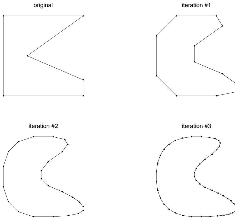
Figure 3.1. Chaikin's algorithm
