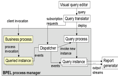
Figure 15: Architecture.
