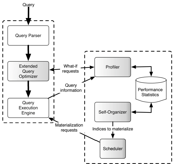
Figure 1. Architecture of COLT.
