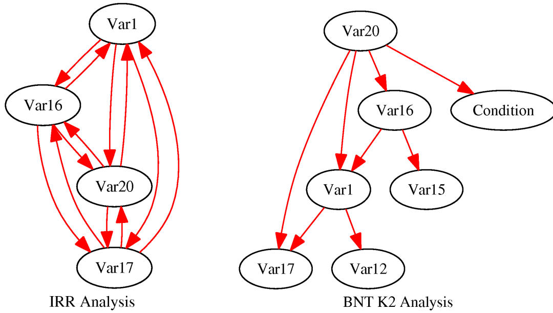
Figure 5: Graphical result of pattern locating. The pattern contains 4 variables (Var1, Var16, Var17, Var20) in a 20 random variables data set. The IRR has fully located the induced pattern, while the BNT has also located two randomly correlated variables (Var12, Var15), not associated in the pattern under the condition.
