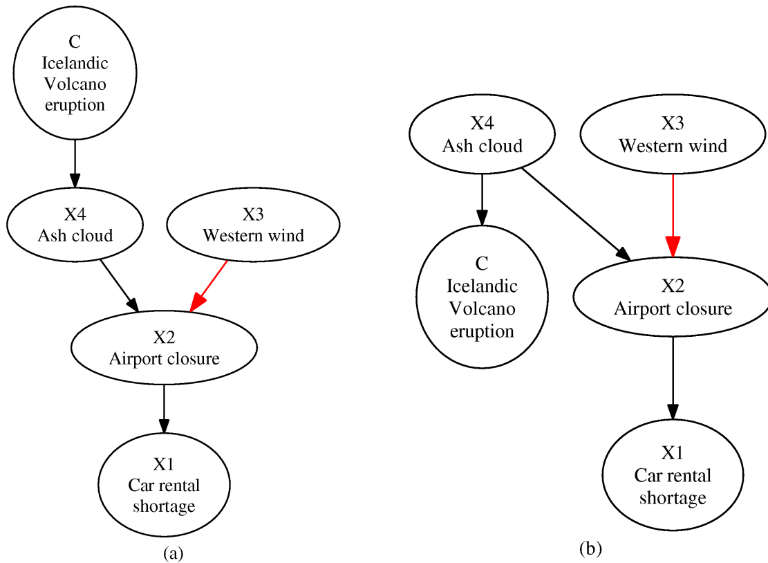
Figure 3 – Alternate Bayesian Network representation of our data. These networks maintain the d-separation criteria between the variables, though now the novel conditioned association ( x_3 \rightarrow x_2 ) should be searched within the whole connected component containing C.
