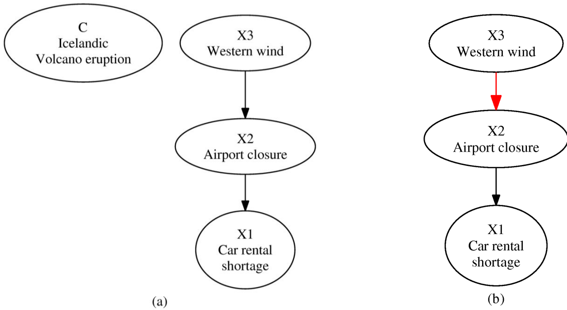
Figure 1 – Graphical representation of the dependencies between three random variables. (a) is the general case and (b) cases under the condition c (Icelandic Volcano eruption) . The edge x_3 \rightarrow x_2 is unique to cases under Condition c.
