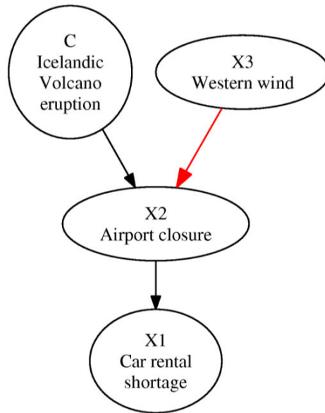
Figure 2 – Bayesian Network representing the joint distribution mapping of X1, X2, X3 and the condition C. The edge x_3 \rightarrow x_2 was retrieved using the BNT.
