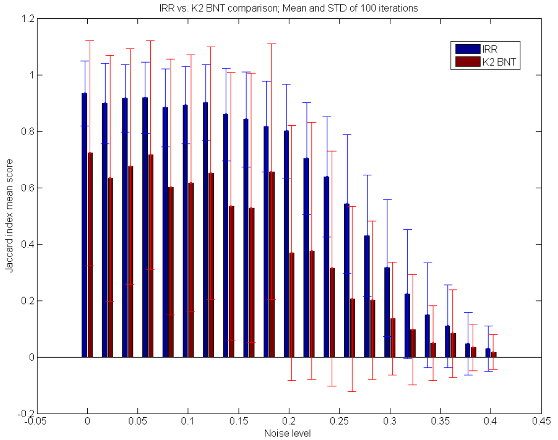
Figure 4: Graphic representation of the Jaccard index scoring mean and STD of the IRR and Bayesian Network K2 algorithms, over 100 iterations. The IRR algorithm significantly outperforms the Bayesian Network K2 algorithm ( p < 0.01 ). The STD values show more stable performance by the IRR as compared with the K2 algorithm.
