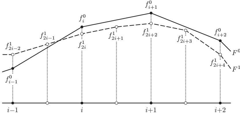
Figure 1: Primal parameterization.
