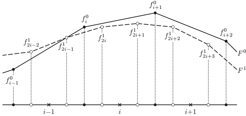
Figure 2: Dual parameterization.
