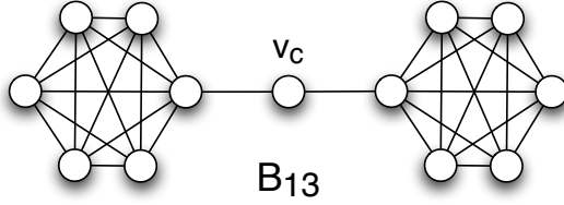
Figure 2: Example barbell graph B_{13} , v_c is the center of the bar-ball
