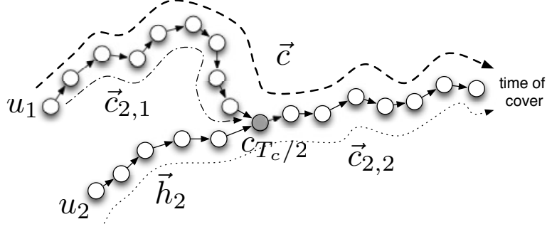
Figure 1: Example for the proof of Lemma 15 with k = 2 . The second walk (dotted line) crosses the last vertex (gray vertex) of the first walk (dash-dot-dash line) and continues in generating a long walk (dashed line) that covers the graph.
