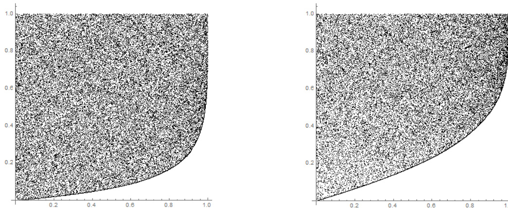
FIGURE 2. The scaled plots of \mathcal{F}^{\text{ddes}}\text{-sort}(\pi) (left) and \mathcal{F}^{\text{val}}\text{-sort}(\pi) (right), where \pi is a permutation chosen uniformly at random from S_{50000} .
