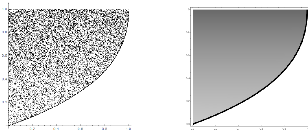
FIGURE 1. On the left is the scaled plot of \text{runsort}(\pi) , where \pi is a permutation chosen uniformly at random from S_{50000} . On the right is the \text{runsort} permuton \mathbf{R} . The dark curve \mathcal{C} is the support of the singular continuous part of \mathbf{R} . Shading within the region \mathcal{C}^+ indicates the density of the absolutely continuous part of \mathbf{R} .
