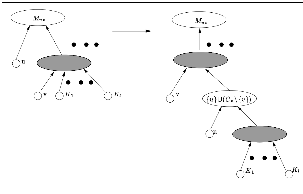
Fig. 1. The updates to the modular decomposition tree in case M_{uv} and C_v have more than two children each, and |C_u| = 1 . Series nodes are drawn shaded.
