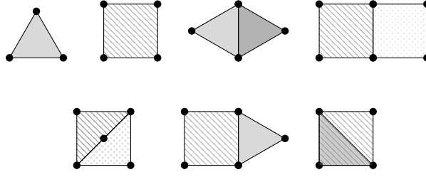
FIGURE 4. The irreducible \{K_3, C_4\} -complexes of size at most two. Copies of K_3 are represented by the grey triangles and copies of C_4 by the hatched or dotted 4-cycles.
