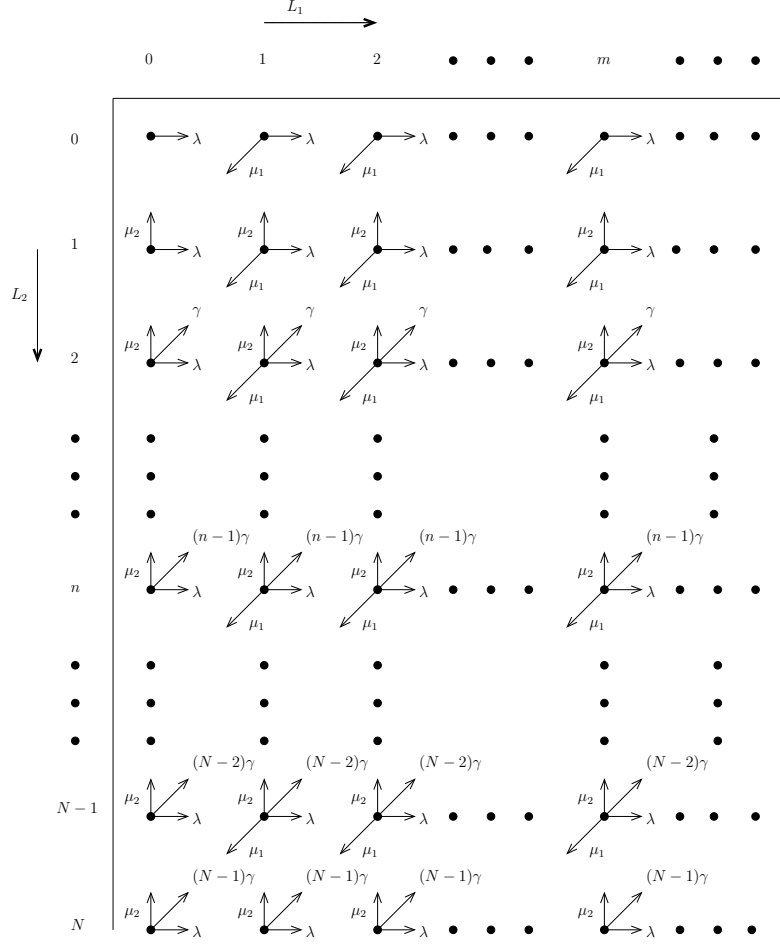
Fig. 2 Transition-rate diagram for (L_1, L_2) .
