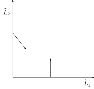
Fig. 4 The state space and directions of reflection for \tilde{L} .
