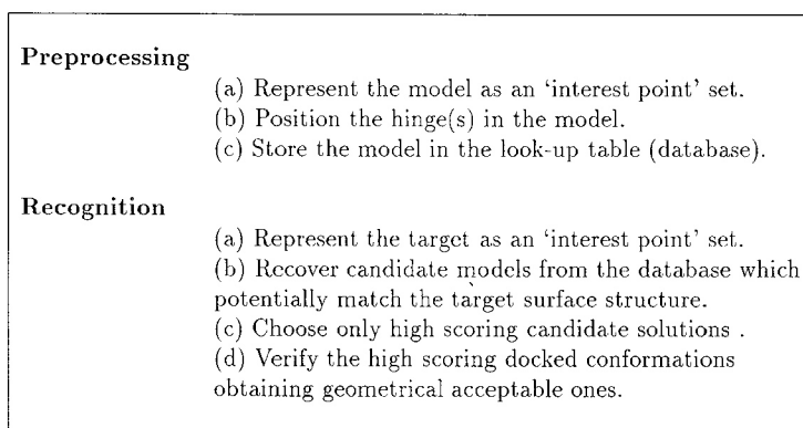
FIG. 2. A general outline of the algorithm. The "model" entity represents the molecular structure of a ligand (or a receptor). The "target" entity represents a receptor (or a ligand) onto which the model(s) are docked. The preprocessing phase can be carried out offline for each new model stored.
