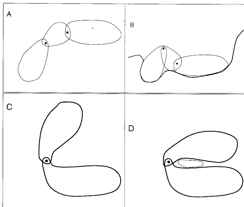
FIG. 1. A schematic illustration of hinge-bending. (A) A flexible ligand consisting of three rigid parts connected by two hinges; two consecutive parts share a common hinge. (B) The flexible ligand displayed in A is docked to a receptor (bold-faced line type). (C) A flexible receptor consisting of two rigid domain parts connected by a hinge—"open form." (D) The flexible receptor displayed in C binds a ligand (light line type)—"closed form."
