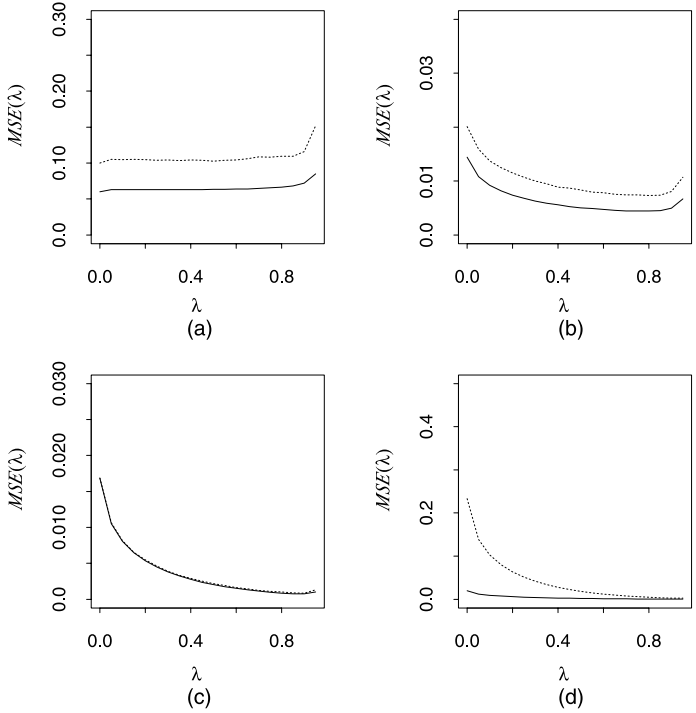
Fig. 5. Plots of MSE(\lambda) versus \lambda for \Gamma = [2, \infty) for (a) \pi_0 = 1 , (b) \pi_0 = 0.8 , (c) \pi_0 = 0.5 and (d) \pi_0 = 0.2 (—, true mean-squared error; ·····, mean-squared error predicted by the bootstrap procedure averaged over 100 applications)
