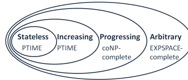
Fig. 1: Middlebox hierarchy.
